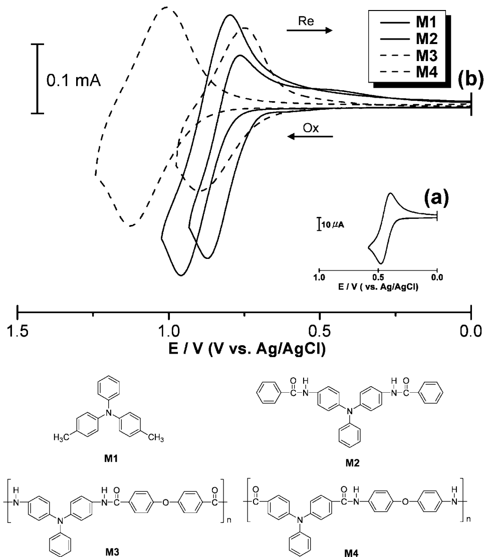
Figure 6. Cyclic voltammograms of (a) ferrocene and (b) model compounds M1 and M2 and polyamides M3 and M4 in \text{CH}_3\text{CN} containing 0.1 M TBAP at scan rate = 0.05 V/s.
