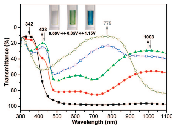
Figure 7. Electrochromic behavior of polyamide 1b thin film (in \text{CH}_3\text{CN} with 0.1 M TBAP as the supporting electrolyte) at (■) 0.00, (●) 0.75, (▲) 0.85, (□) 0.95, and (○) 1.15 V vs Ag/AgCl. 1b + , solid symbols with black arrows; 1b 2+ , open symbols with gray arrows.
